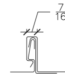
SNAP LOCK CLIPS
